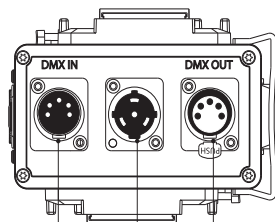
DMX IN Port NEUTRIK powerCON Power Input DMX OUT Port
